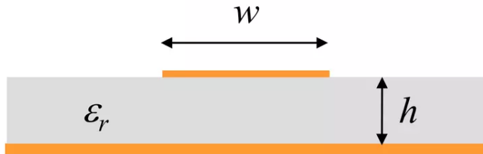
Microstrip
