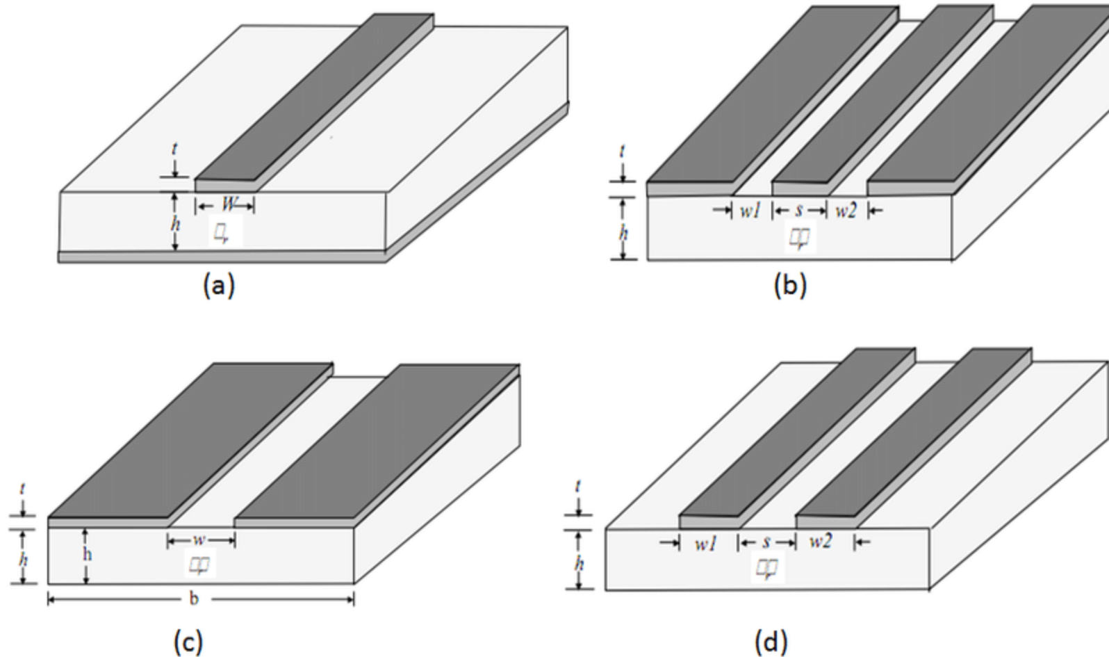
Types of planar TLs [1]: (a) microstrip; (b) coplanar waveguide, (c) slot line, and (d) coplanar strip line
