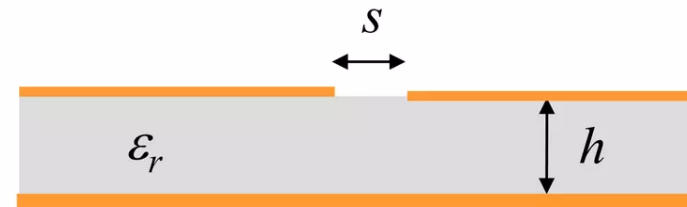
Conductor-backed Slotline
