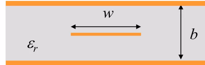
Stripline
